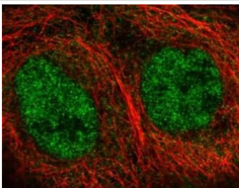
Immunofluorescent analysis of A431 cells labeling FAM63A with ab220932 at 4 µg/mL (green).
