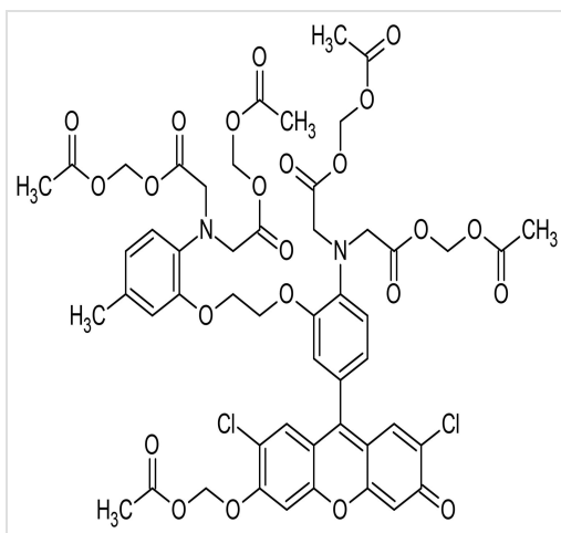
Chemical Structure - Fluo-3 AM, Fluorescent calcium Indicator (ab145254)
