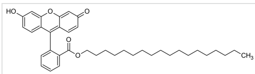
Chemical Structure - Fluorescein octadecyl ester, Lipophilic fluorescent pH indicator (ab145431)
