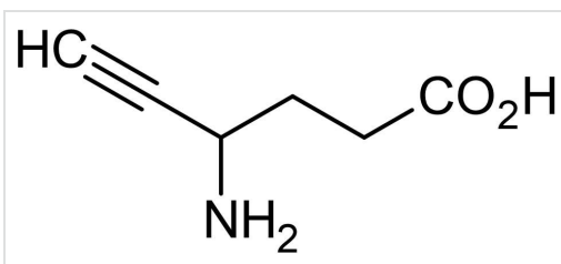
2D chemical structure image of ab145973, gamma-Acetylenic GABA, GABA transaminase inhibitor
