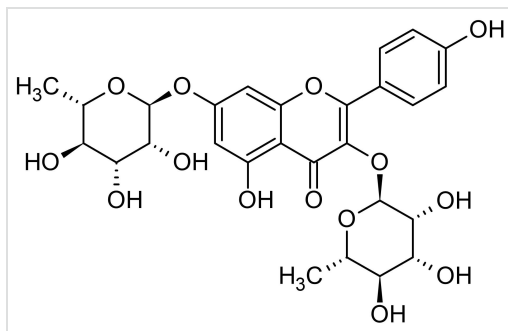
Chemical Structure - Kaempferitrin (Lespenefril), Antioxidant agent (ab144286)
