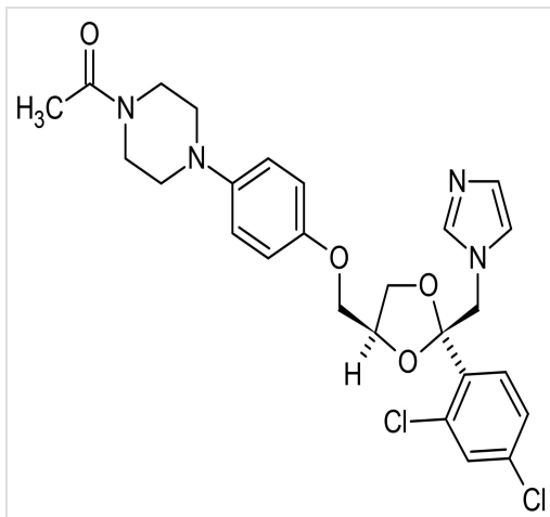
Chemical Structure - Ketoconazole, cytochrome P450 inhibitor (ab120620)
