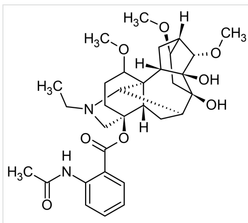
Chemical Structure - Lappaconitine, analgesic agent (ab143507)
