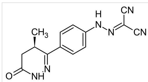
Chemical Structure - Levosimendan, phosphodiesterase inhibitor (ab142315)
