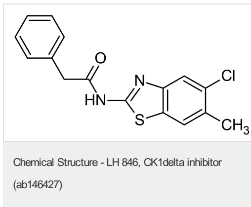
2D chemical structure image of ab146427, LH 846, CK1delta inhibitor
