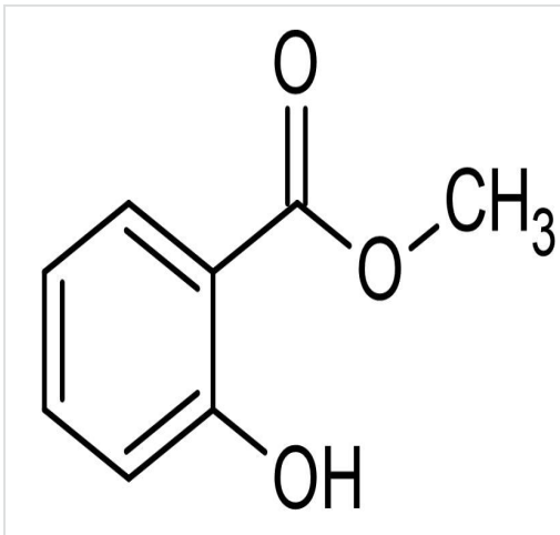
2D chemical structure image of ab142913, Methyl salicylate, Salicylic acid analog
