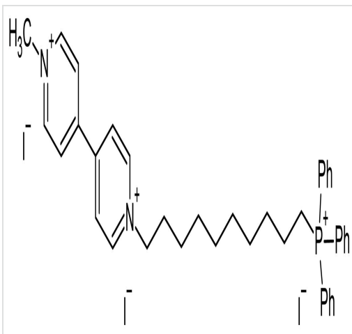
Chemical Structure - MitoPQ, mitochondria-targeted redox cyclers (ab146819)
