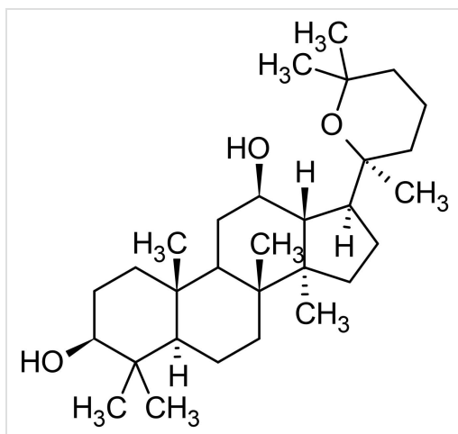
Chemical Structure - Panaxadiol, Anticancer agent (ab142336)
