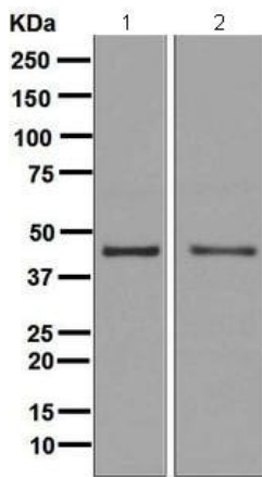
Western blot - Anti-PDCD2 antibody [EPR7159] (ab126614)
