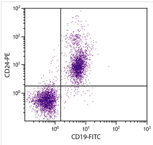
Flow Cytometry - PE Anti-CD24 antibody [30-F1] (ab25494)
