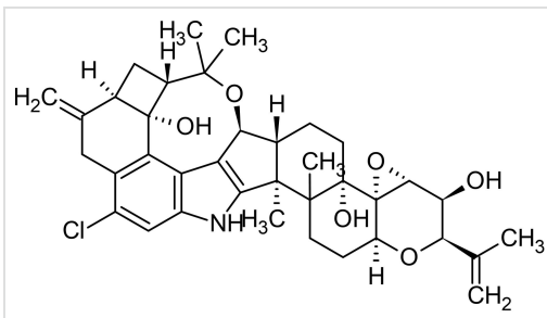
Chemical Structure - Penitrem A, blocker of KCa1.1 (ab141842)
