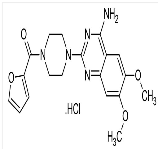
Chemical Structure - Prazosin hydrochloride, Peripheral alpha adrenoceptor antagonist (ab120238)
