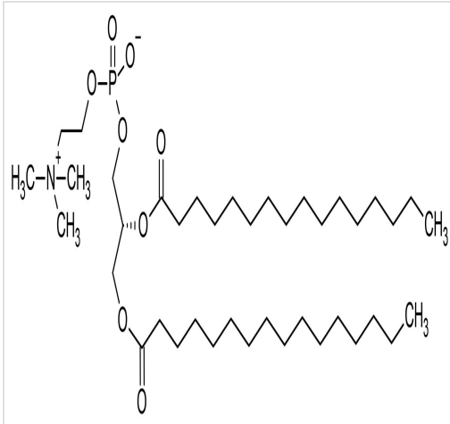
Chemical Structure - 1,2-Dipalmitoyl-sn-glycero-3-phosphorylcholine (DPPC), Phosphatidylcholine (ab143947)
