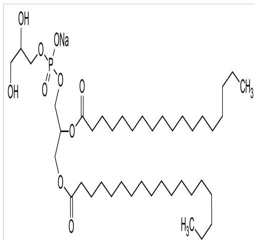
Chemical Structure - 1,2-Distearoyl-sn-glycero-3-phosphorylglycerol sodium salt (DSPG), Phosphorylglycerol (ab143954)
