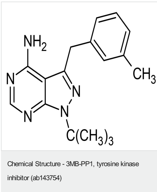
2D chemical structure image of ab143754, 3MB-PP1, tyrosine kinase inhibitor
