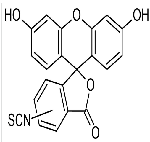
2D chemical structure image of ab145258, 5(6)-FITC (Fluorescein 5(6)-isothiocyanate), Fluorescent amine-reactive label
