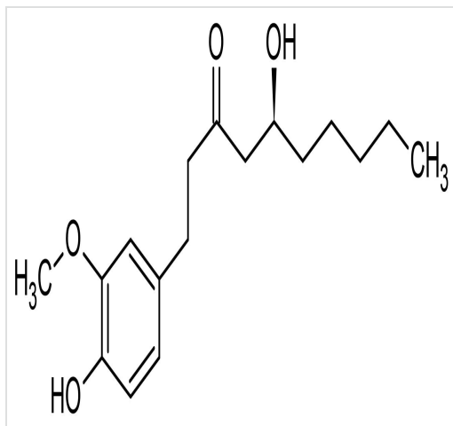
Chemical Structure - 6-Gingerol, Anti-inflammatory agent (ab145635)
