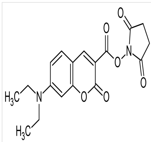
Chemical Structure - 7-Diethylaminocoumarin-3-carboxylic acid N-succinimidyl ester, Fluorescent labeling reagent (ab145264)
