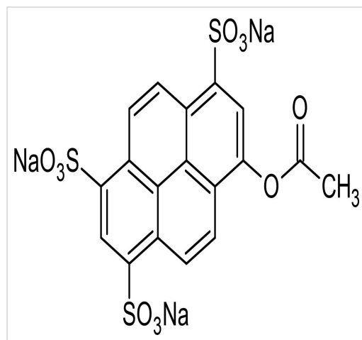
Chemical Structure - 8-Acetoxypyrene-1,3,6-trisulfonic acid trisodium salt, Fluorogenic esterase substrate (ab145400)
