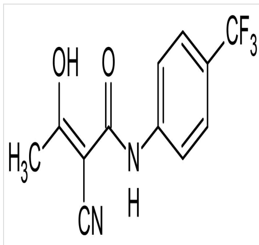
Chemical Structure - A771726 (Teriflunomide), Active metabolite of leflunomide. Dihydroorotate dehydrogenase inhibitor. (ab141480)
