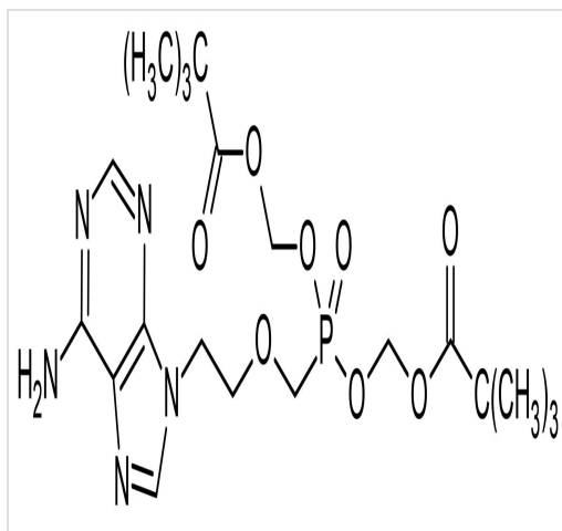
Chemical Structure - Adefovir Dipivoxil (bis-POM PMEAs), nucleotide analog reverse transcriptase inhibitor (ab143063)
