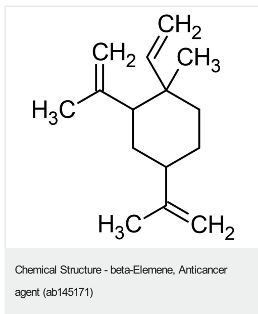
2D chemical structure image of ab145171, beta-Elemene, Anticancer agent
