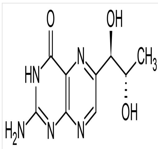
Chemical Structure - Biopterin, coenzyme and cofactor of iNOS activity (ab142835)
