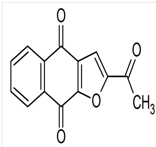
Chemical Structure - Cancer cell stemness inhibitor (Napabucasin), high-cancer cell inhibitor (ab145630)
