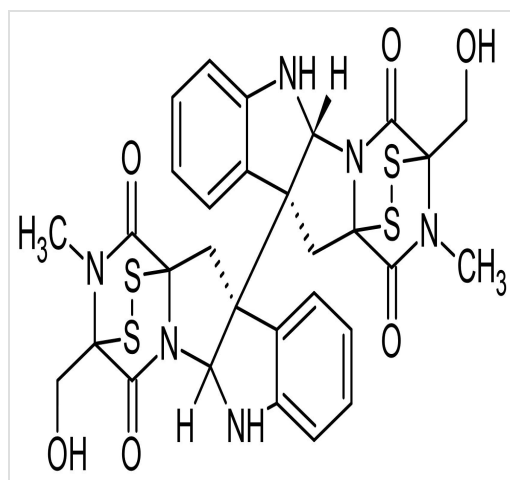
Chemical Structure - Chaetocin, histone lysine methyltransferase inhibitor (ab144534)
