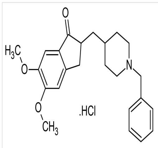
Chemical Structure - Donepezil hydrochloride, Acetylcholinesterase inhibitor (ab120763)
