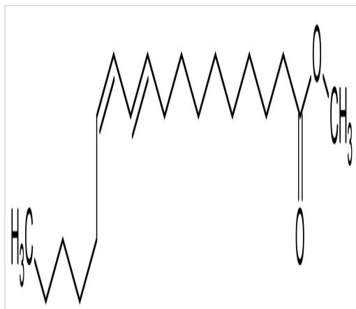
Chemical Structure - Methyl 10(E), 12(Z)-octadecadienoate, Conjugated linoleic acid methyl ester (ab143918)
