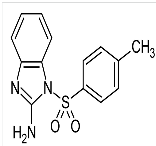
Chemical Structure - ML130, NOD1 inhibitor (ab142177)
