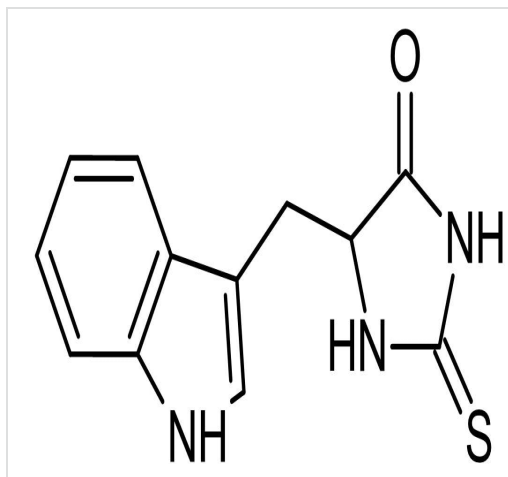
Chemical Structure - Necrostatin-1, inactive control, N-demethylated thiohydantoin analog of Necrostatin- 1 (ab145889)
