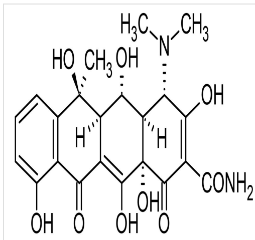
Chemical Structure - Oxytetracycline, Tetracycline antibiotic (ab143429)
