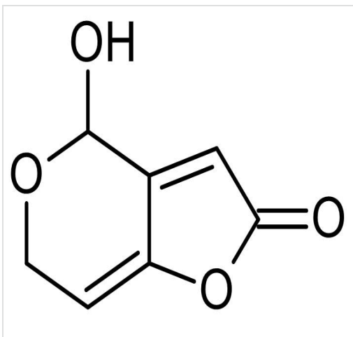
Chemical Structure - Patulin, fungal mycotoxin (ab142725)
