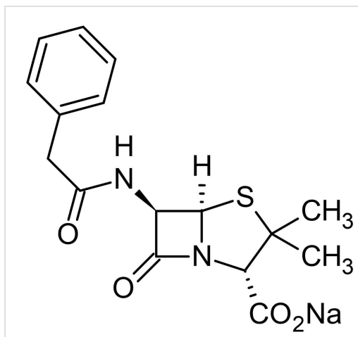
2D chemical structure image of ab145634, Penicillin G sodium (Benzylpenicillin sodium), beta-lactam antibiotic agent
