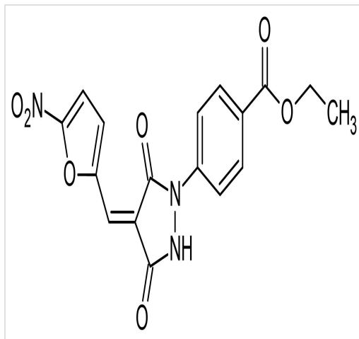
Chemical Structure - PYR-41, Ubiquitin-activating enzyme (E1) inhibitor (ab141469)
