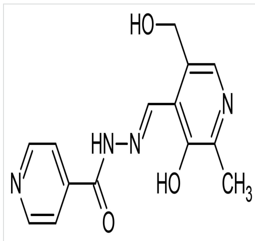
Chemical Structure - Pyridoxal isonicotinoyl hydrazone (PIH), hydrazone iron chelator (ab145871)
