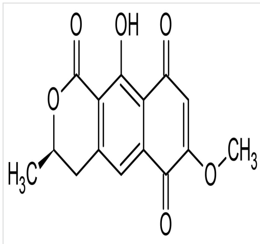
Chemical Structure - (R)-Semixanthomegnin, mycotoxin derivative (ab144360)
