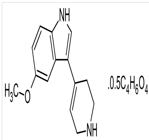
Chemical Structure - RU 24969 hemisuccinate, 5-HT 1A/1B agonist (ab146299)
