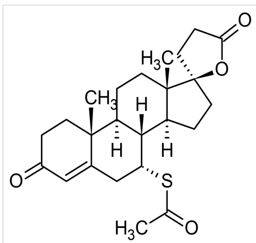
Chemical Structure - Spironolactone, Mineralocorticoid receptor antagonist (ab141289)
