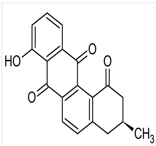
Chemical Structure - STA-21 (Ochromycinone), STAT3 inhibitor (ab145648)
