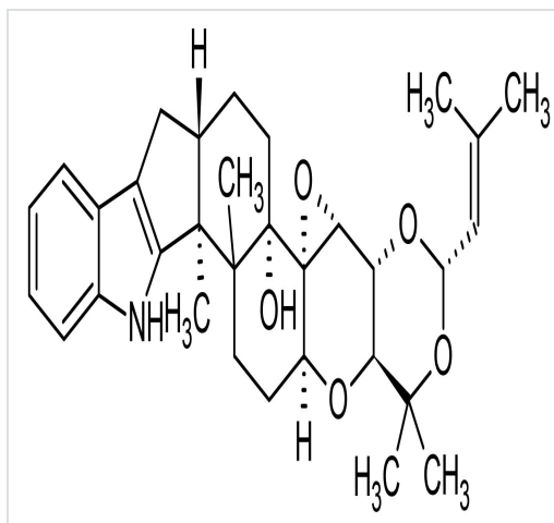
Chemical Structure - Terpendole C, ACAT1 and ACAT2 inhibitor (ab144367)
