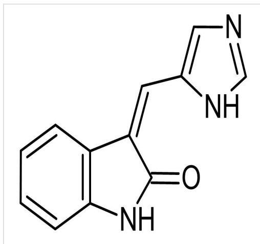
Chemical Structure - Tripolin B, Aurora A and B inhibitor (ab144378)
