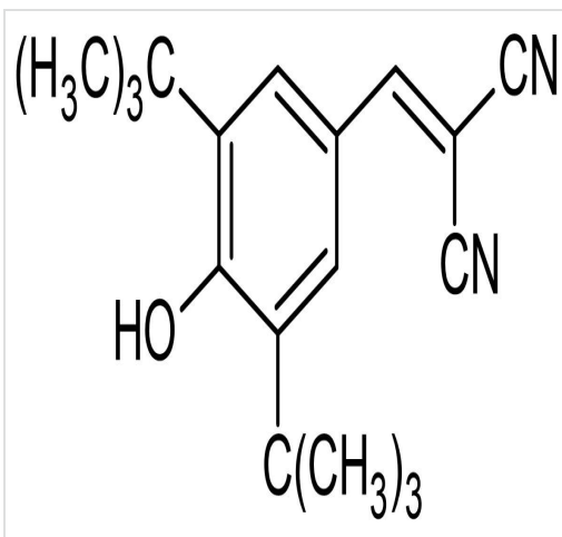
Chemical Structure - Tyrphostin 9, PDGFR tyrosine kinase inhibitor (ab141561)
