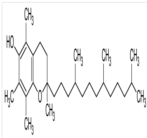
Chemical Structure - Vitamin E (DL-alpha-Tocopherol), Fat-soluble antioxidant (ab142968)
