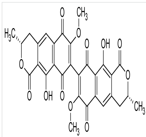
Chemical Structure - Xanthomegnin, iNOS inhibitor (ab144386)
