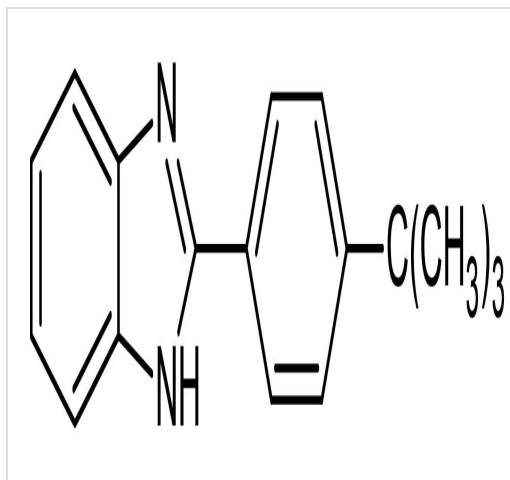
Chemical Structure - ZLN005, PGC-1alpha transcriptional activator (ab145641)
