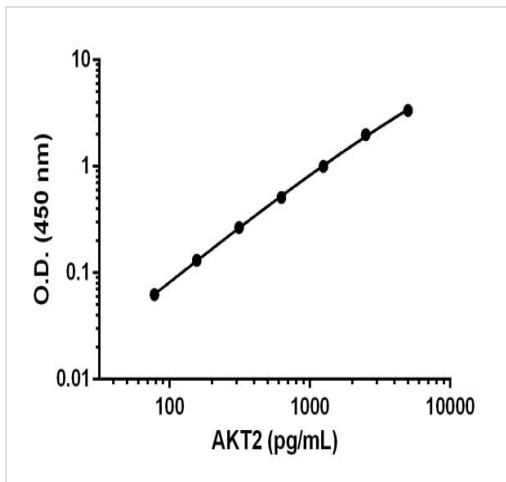
Sandwich ELISA - Mouse AKT2 Antibody Pair - BSA and Azide free (ab241767)
