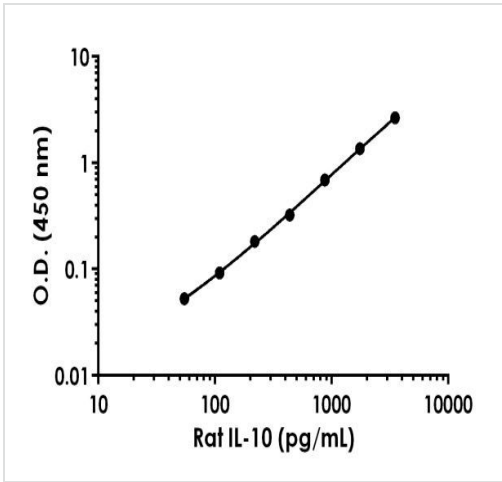
Representative standard curve from corresponding SimpleStep ELISA® Kit ( ab214566 ).
